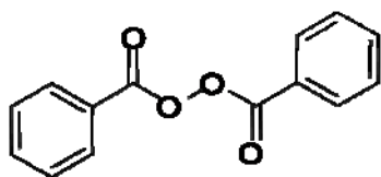
Benzoyl Peroxide:
